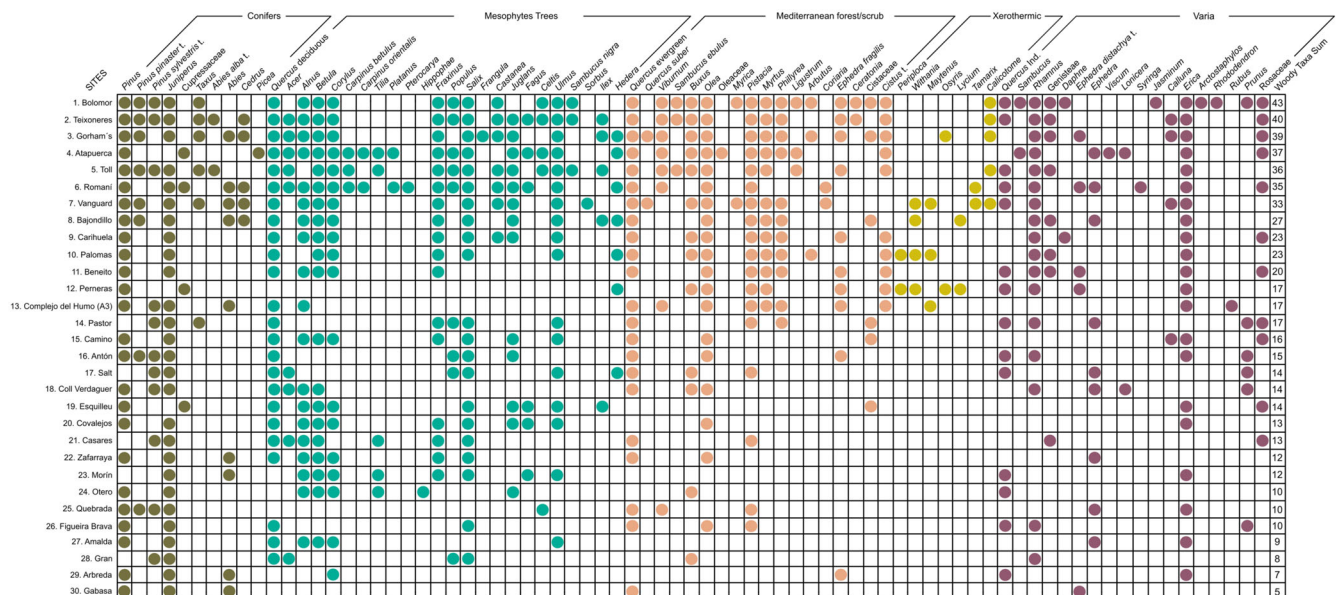
Figure 9. Woody taxa and their ecological categories in palynological sequences from Iberian Neanderthal sites. [Color figure can be viewed at wileyonlinelibrary.com ] [3005/2024]. See the Terms and Conditions ( https://onlinelibrary.wiley.com/terms-and-conditions ) on Wiley Online Library for rules of use. OA articles are governed by the applicable Creative Commons License
