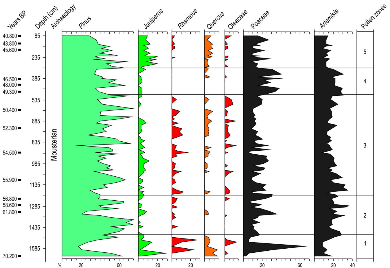
Figure 10. Main pollen curves and chronology of the Upper Pleistocene Romaní cave sequence (Burjachs and Julià, 1994). [Color figure can be viewed at wileyonlinelibrary.com ] [3005/2024]. See the Terms and Conditions ( https://onlinelibrary.wiley.com/terms-and-conditions ) on Wiley Online Library for rules of use. OA articles are governed by the applicable Creative Commons License
