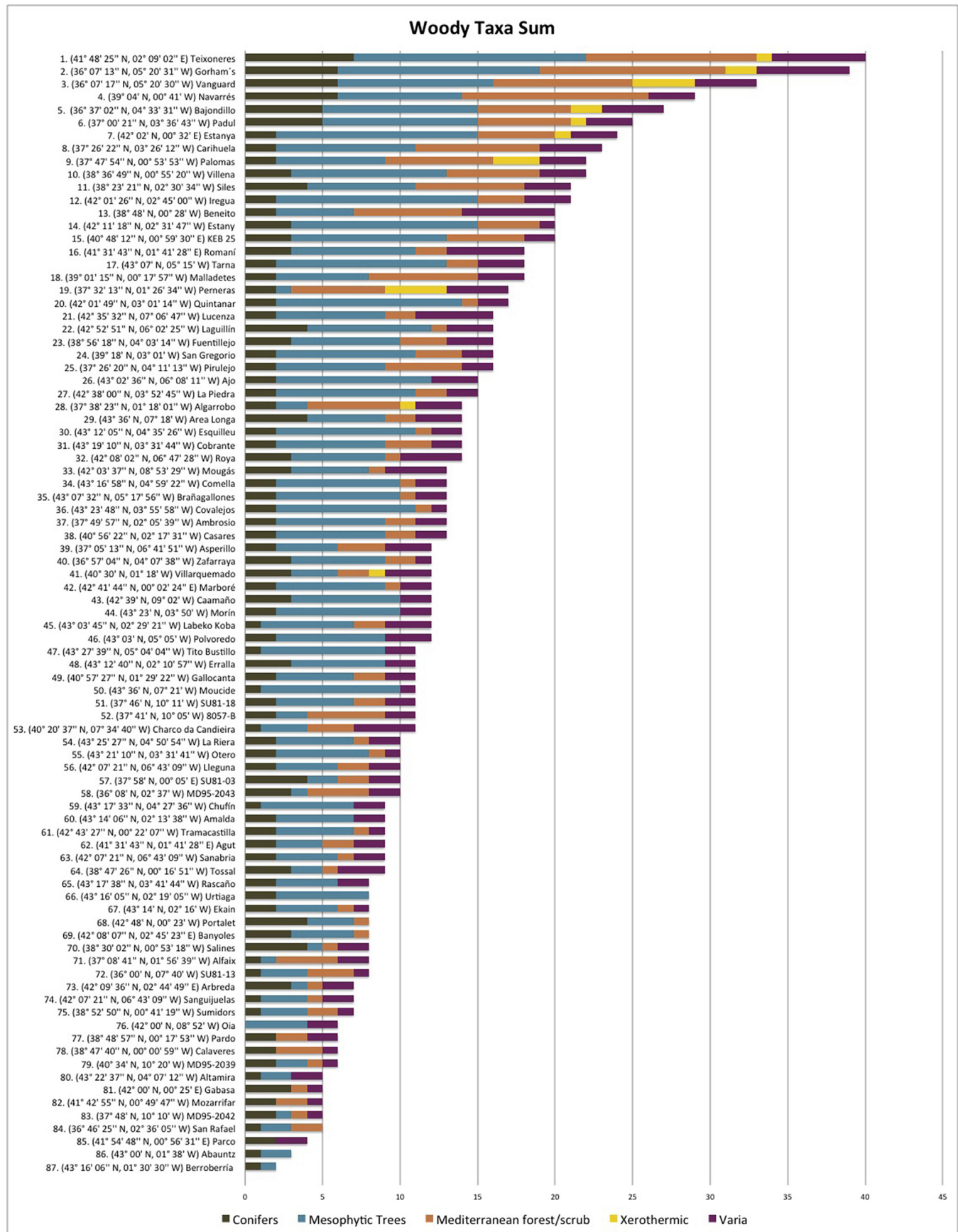
Fig. 9. Number of woody taxa, conifers, mesophytes, Mediterranean and xerothermics in Quaternary palaeoecological sequences of the Iberian Peninsula for the MIS 3-2 interval. Teixoneres arises as the site with highest woody taxa diversity. Data obtained from Carrión et al. (2013) .
