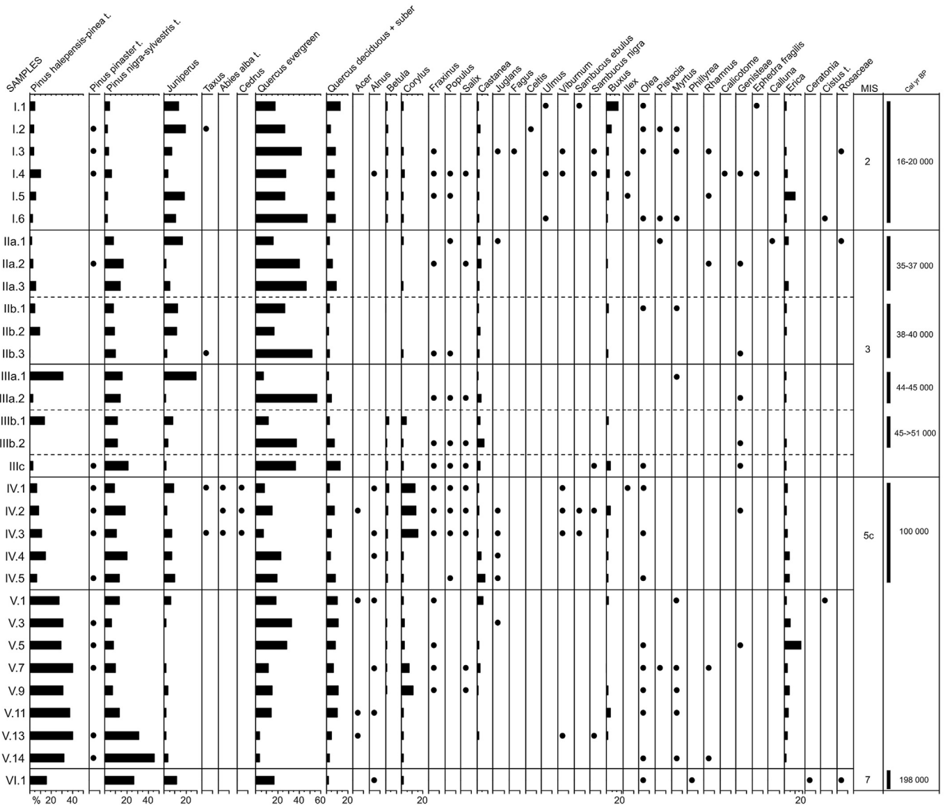
Fig. 3. Pollen diagram of Teixoneres including principally the woody component. Black dots for percentages below 3%. Dashed lines for subdivisions within archaeological levels.
