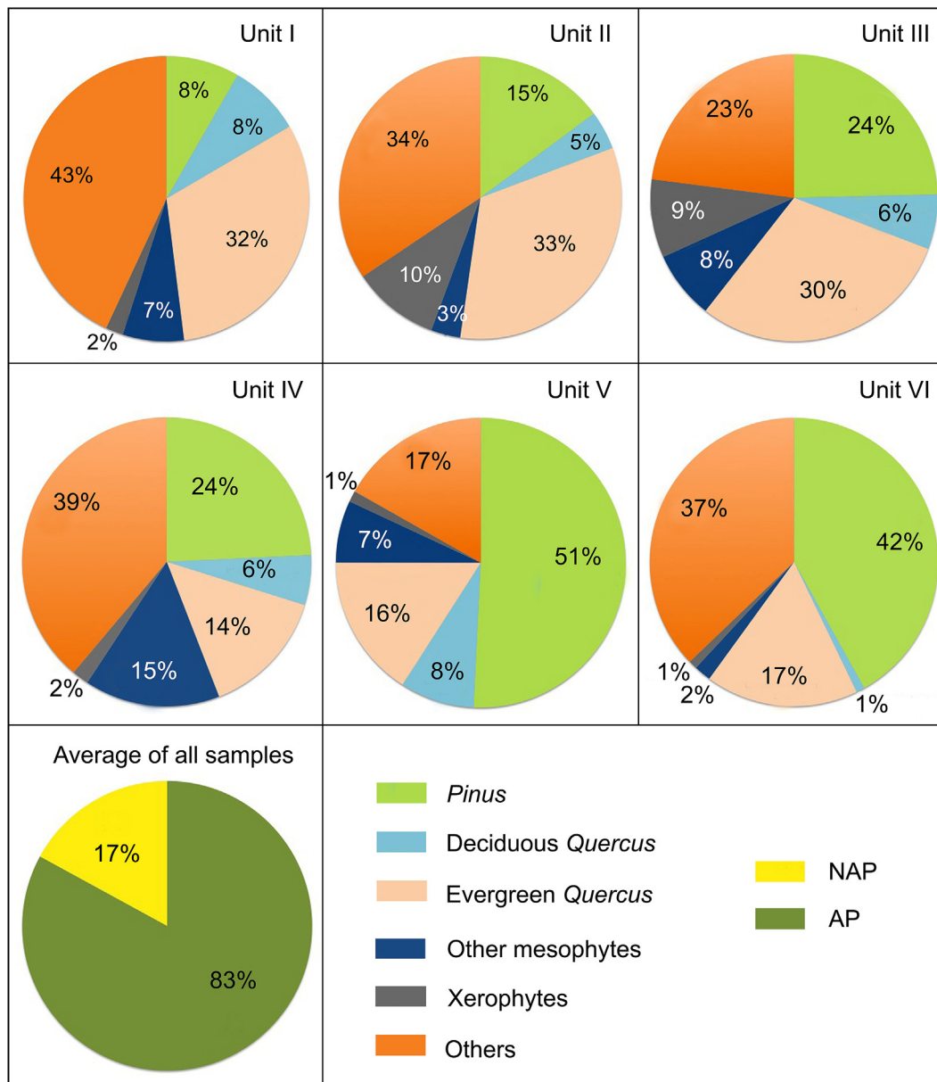
Fig. 6. Sum of pollen frequencies for selected taxa and pollen groups, including arboreal (AP) and non-arboreal (NAP) components in the sequence of Teixonerres.
