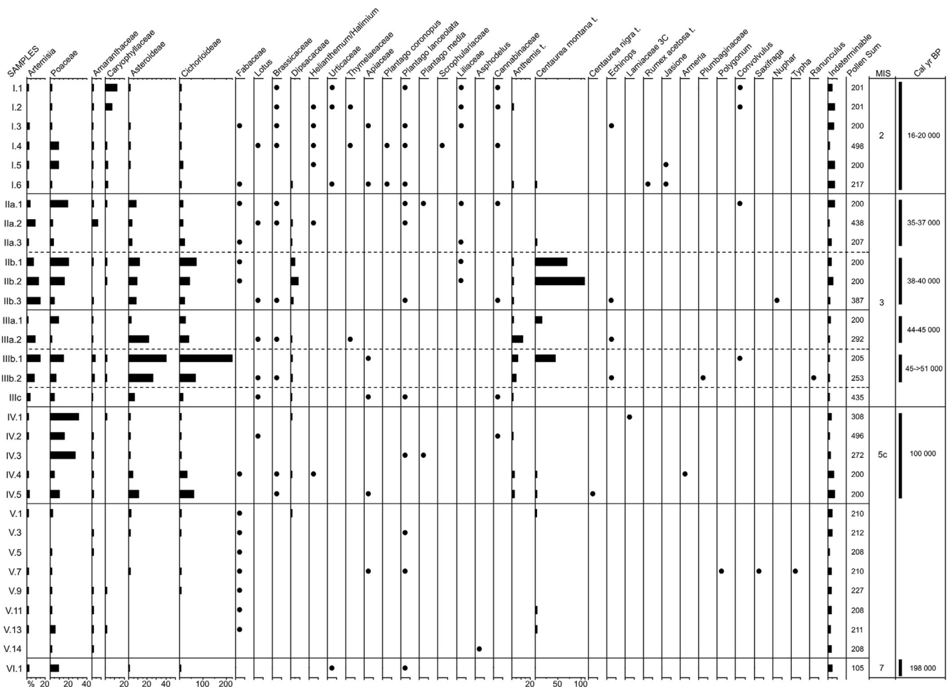
Fig. 4. Pollen diagram of Teixoneres including mainly non arboreal elements. Asteroideae, Cichorioideae, Anthemis type, Centaurea montana type, Centaurea nigra type and Echinops are out from the total pollen sum. Black dots for percentages below 3%. Dashed lines for subdivisions within archaeological levels.
